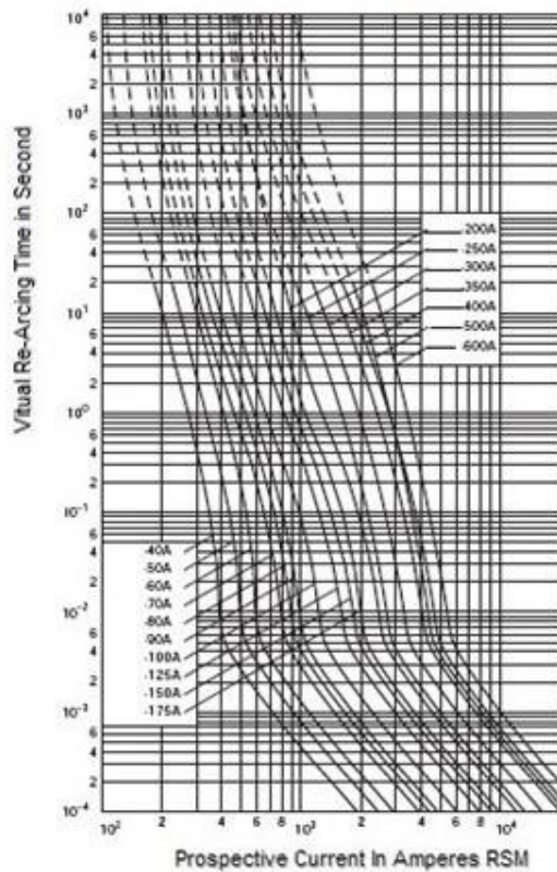
Time-Current Curve 40A-600A/1000V
