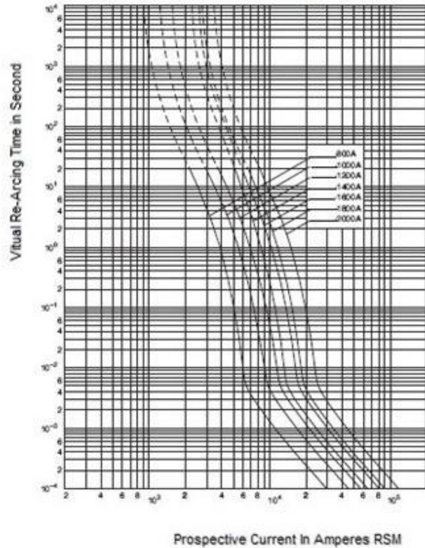
Time-Current Curve 800A-2000A/1000V
